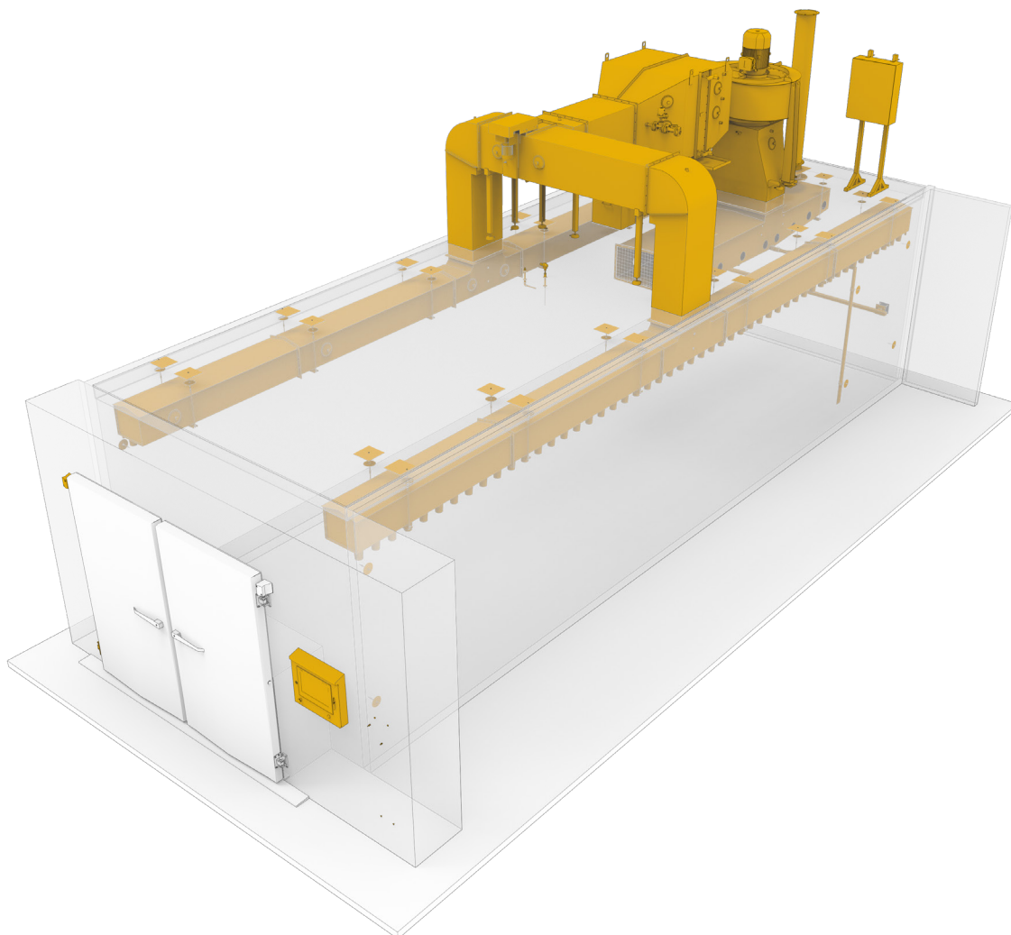
Fig. 1 CLIMAMAT DEFROST
